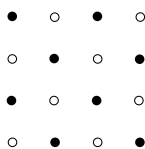
FIGURE 1. Staggered array of point vortices (● = positive, ○ = negative) in a single grid box used as the initial conditions. The vortices are separated by \Delta x/4 both horizontally and vertically, where \Delta x is the grid size.
